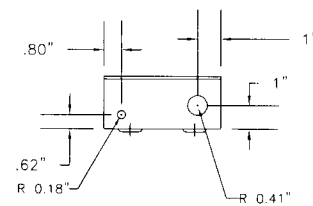
TOP DETAIL
