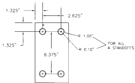
STANDOFF DETAIL
